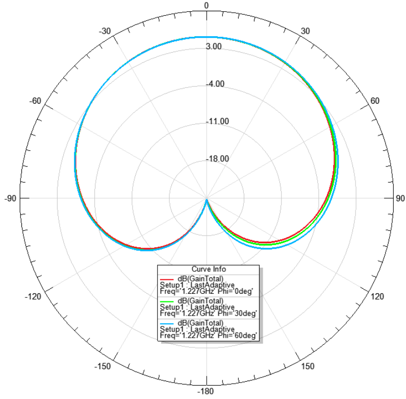
Gain Plot 2
